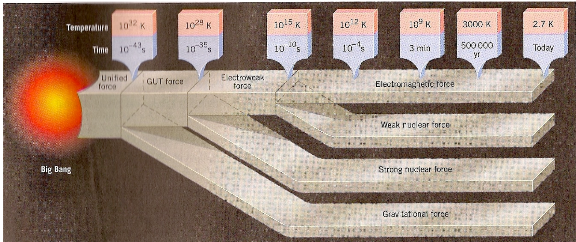
Figure 32.16 According to the standard cosmological model, the universe has evolved as illustrated here. In this model, the universe is presumed to have originated with a cataclysmic event known as the Big Bang. The times shown are those following this event.
